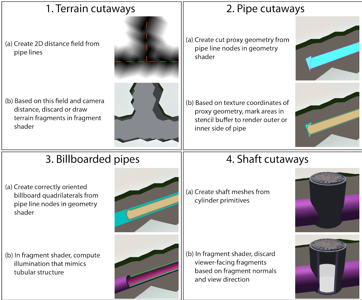
Fig. 3. Overview diagram of the presented approach.
