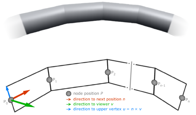
Fig. 7. Arrangement of quadrilaterals in a billboarded pipe. Quadrilateral vertices are constructed based on the pipe line nodes and the view direction.
